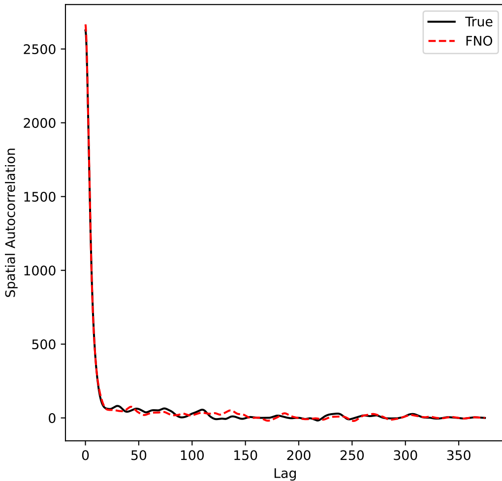
Autocorrelation Comparison with MSE = 2.6 \times 10^2
