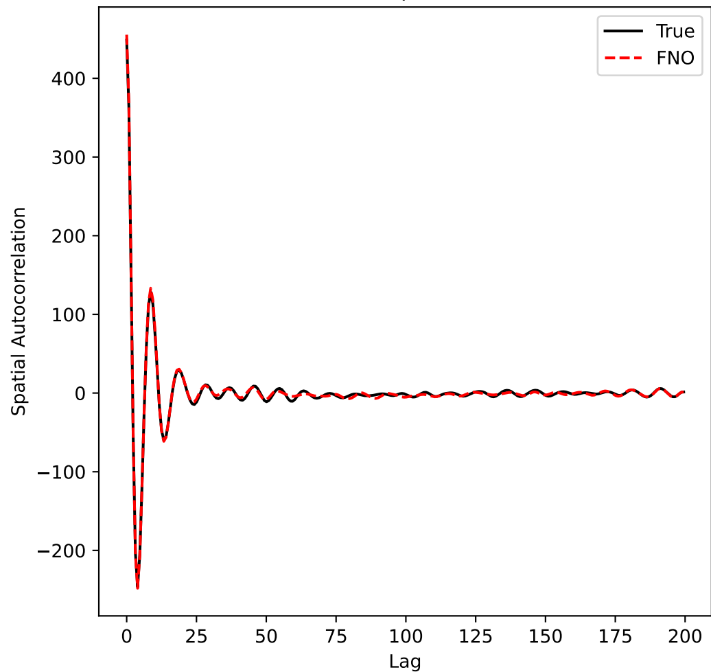
Autocorrelation Comparison with MSE = 5
