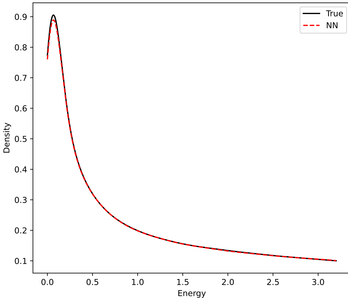
TKE Density Comparison with KS: 0.005, p-value: 2.5e-34
